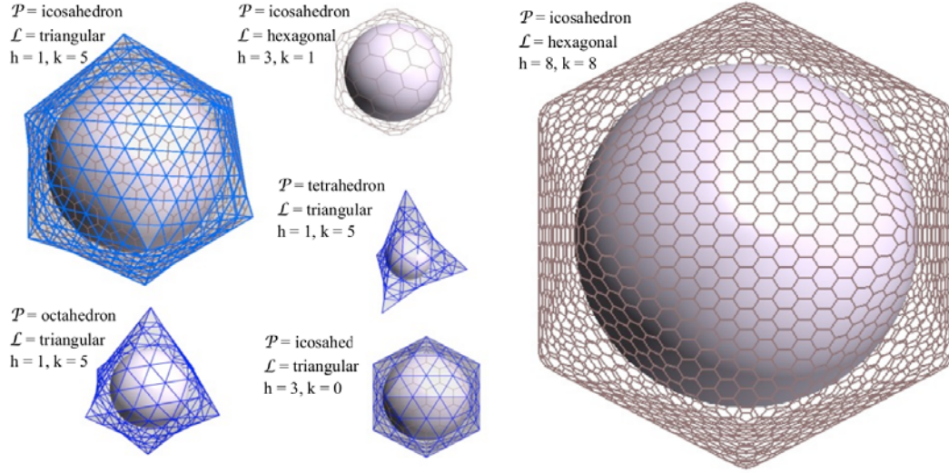
Fig. 8. Some polyhedron generated by applying Til ingGen.
