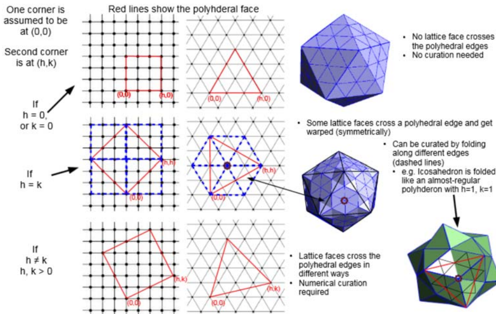
Fig. 9. Different cases of warping of tiles, and their curations.
