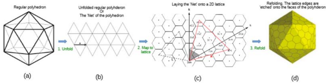
Fig. 5. Illustration of the Goldberg construction. The Goldberg construction involves unfolding an icosahedron (see (a) and (b)), and then mapping the unfolded icosahedron onto a 2D hexagonal lattice scaled and oriented such that all corners of the unfolded icosahedron (its original vertices) fall on the centers of some hexagon of the grid (some example scale and orientations (for one triangle only) are shown (c)). Finally, the icosahedron is folded back, along with the hexagonal grid etched onto its faces. For example, for the scaling and orientation of the red triangle in (c), would result in the tiled icosahedron shown in (d). Notice that the new polyhedron has exactly 12 regular pentagonal faces, where the icosahedral vertices originally were, and many regular hexagonal faces.
