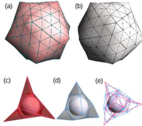
Fig. 10. Numerical curvation of warped faces. Top row: (a) shows a polyhedron with icosahedral symmetry and 260 tiles. The color of the triangles are determined by the ratio of the longest and the shortest edge of the tile. Ratios 1 to 1.3+ are colored using white to red gradient. The triangles at the corners and near the edges of the icosahedron have higher distortion. (b) shows the result of numerical curvation. All the triangles are now regular, the worst ratio being 1.034, and the symmetry is preserved. Bottom row: (c-d) show a similar before-after figure for a smaller polyhedra, but one where the warping is more apparent. The numerical optimization brought down the ratio of the worst triangle from 2.13 to 1.004. (e) shows a superposition of the two states to highlight that points are updated symmetrically.
