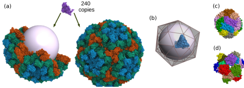
Fig. 1. Motivation for studying congruent meshed polyhedra. (a) Most viruses have a symmetric shell protecting its genome (shown only as a sphere in the figure). The shell is formed by multiple copies of a single building block (protein) arranged symmetrically. (b) The arrangement of the proteins for the virus shown in (a) uniquely maps to a tiled polyhedra with icosahedral symmetry. The polyhedra sufficiently characterizes all relevant symmetry and topology information and serves as a template for the analysis, prediction and construction of such shells. (c-d) Shell structures in nature also comes in octahedral and tetrahedral symmetries. Our class of polyhedra covers all these cases.
