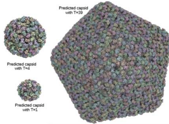
Fig. 13. Shells of different sizes using the same protein
