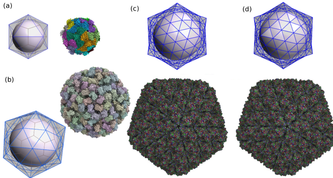
Fig. 12. Predicted shell structures for known viruses. (a) Predicted shell structure for Tobacco Necrosis Virus using a polyhedra with h=1 , k=0 . (b) Predicted shell structure for Nudaurelia Capensis Virus using a polyhedron with h=2 , k=0 . (c) Predicted shell structure for Rice Dwarf Virus outer shell using h=1 , k=3 . (d) Predicted structure for the same virus with h=3 , k=1 . All the predicted models have the correct inter-tile (or inter-protein) interfaces/contact in terms of geometry, and have the correct global and local topology; except, the one in (c) which has wrong chirality).
