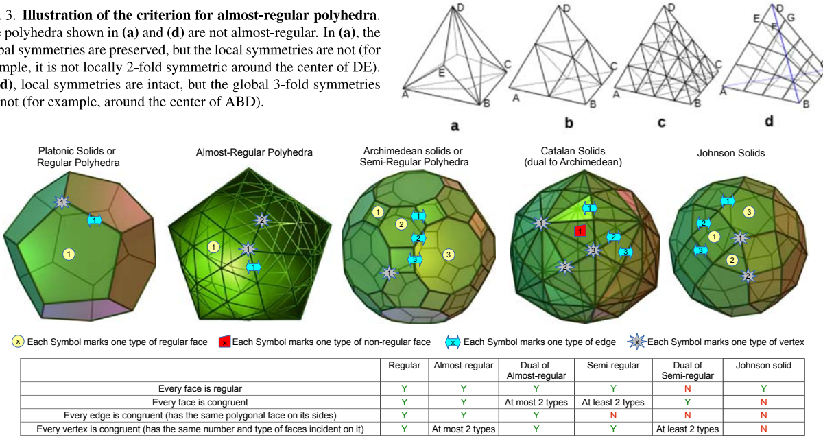
Fig. 4. Illustration of different classes of symmetric polyhedra. We show example polyhedra from regular, almost-regular , semi-regular, duals of semi-regular, and Johnson solids. The table compares the symmetry and congruency properties of the classes. The symbols embedded on the polyhedra show the distinct types of faces/edges/vertices present in them.
