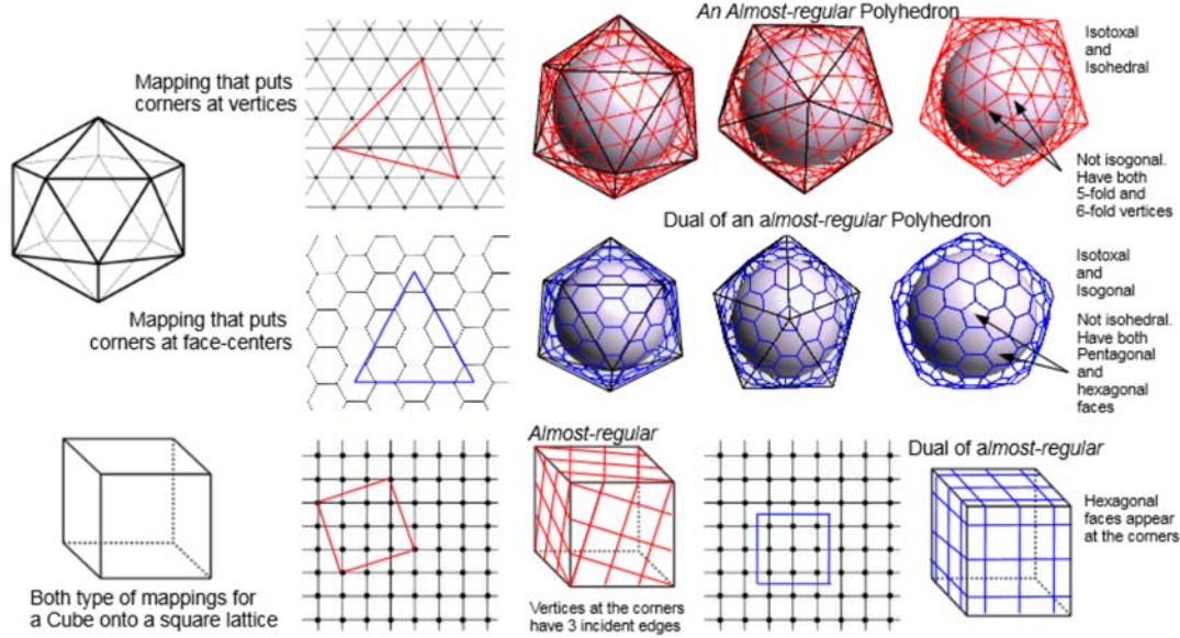
Fig. 7. Illustration of the constructing almost-regular polyhedron and their duals. Top row shows how placing corners of a polyhedral face on vertices of a compatible lattice produces an almost-regular polyhedron. The black lines show the original polyhedron, and the red lines show the etching/tiling induced by the lattice. The second row shows an example of placing the corners at face centers and producing duals of almost-regular polyhedron. Finally, the bottom row shows examples of both the primal and the dual constructions using a square lattice.
