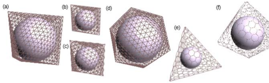
Fig. 2. A small sample from our family of almost-regular polyhedra. The family provides infinite series of polyhedra having the same global and local symmetries, using the same type of tiles and inter-tile matching rule (or edges). For example, (a–c) shows three examples having octahedral symmetries but using 1352, 392 and 504 tiles respectively. This allows the design of progressively finer meshes, or enables templating for larger structures using the same building block. The family also covers multiple types of global symmetries. For example, in (d), we see a mesh with icosahedral symmetry but using almost the same number of tiles as (a). Finally, our construction also supports other regular tilings, for example hexagonal honeycomb tilings shown in (e–f) with tetrahedral and octahedral global symmetries respectively. Note that the examples shown in (a–c) and (e–f) do not fall under the classic Goldberg construction.
